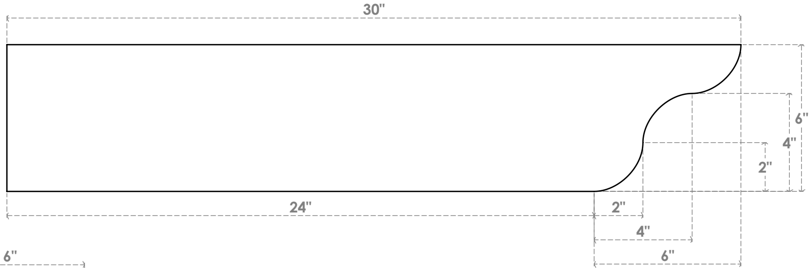
SIDE PROFILE
